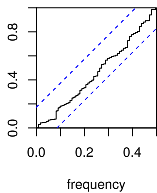
Standardized Residuals
