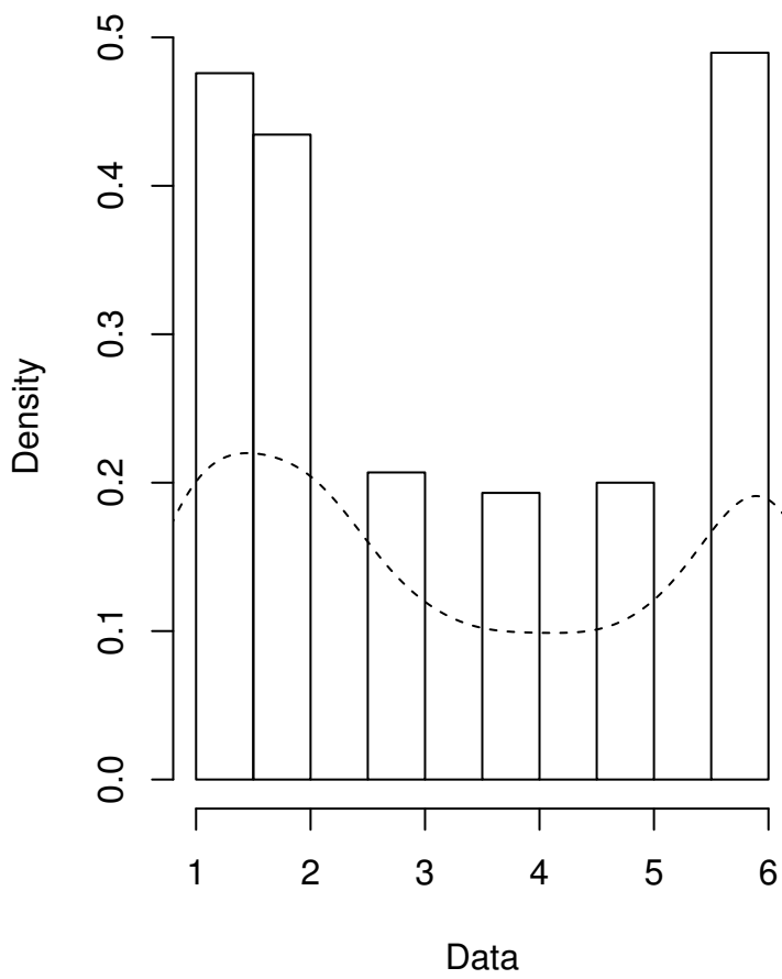
Empirical density
