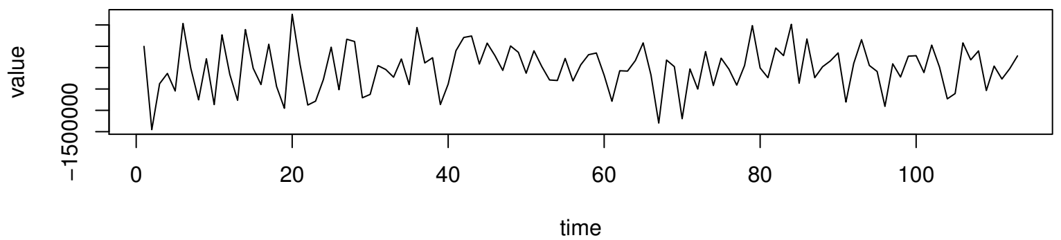
Working Time Series (lambda=1.8, d=1, D=1)
