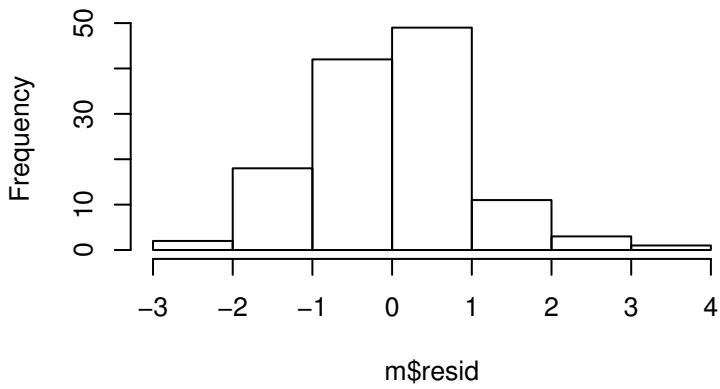
Residual Histogram
