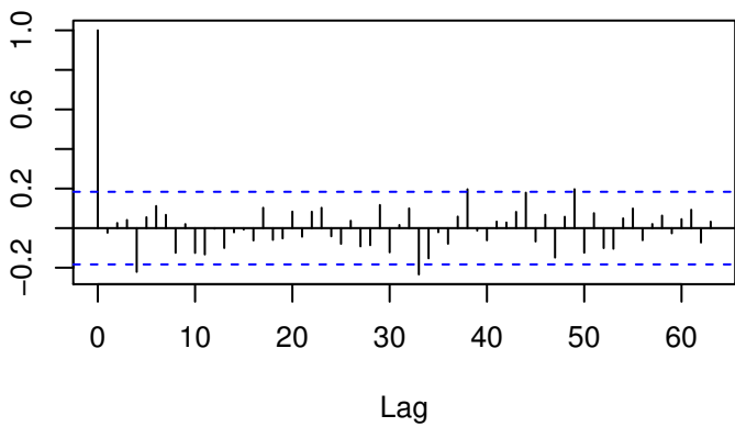
Residual ACF
