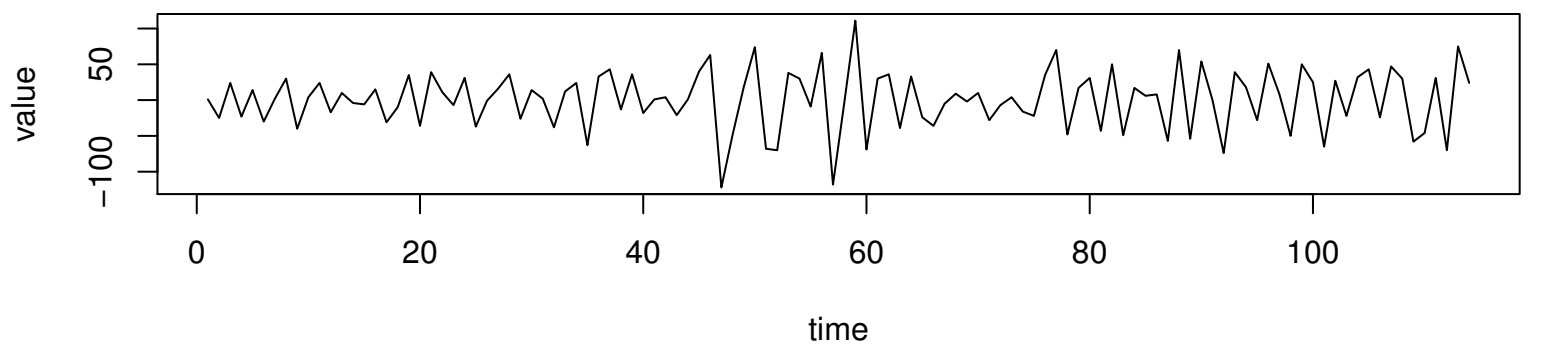
Working Time Series ( \lambda=1 , d=2 , D=0 )
