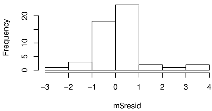
Residual Histogram
