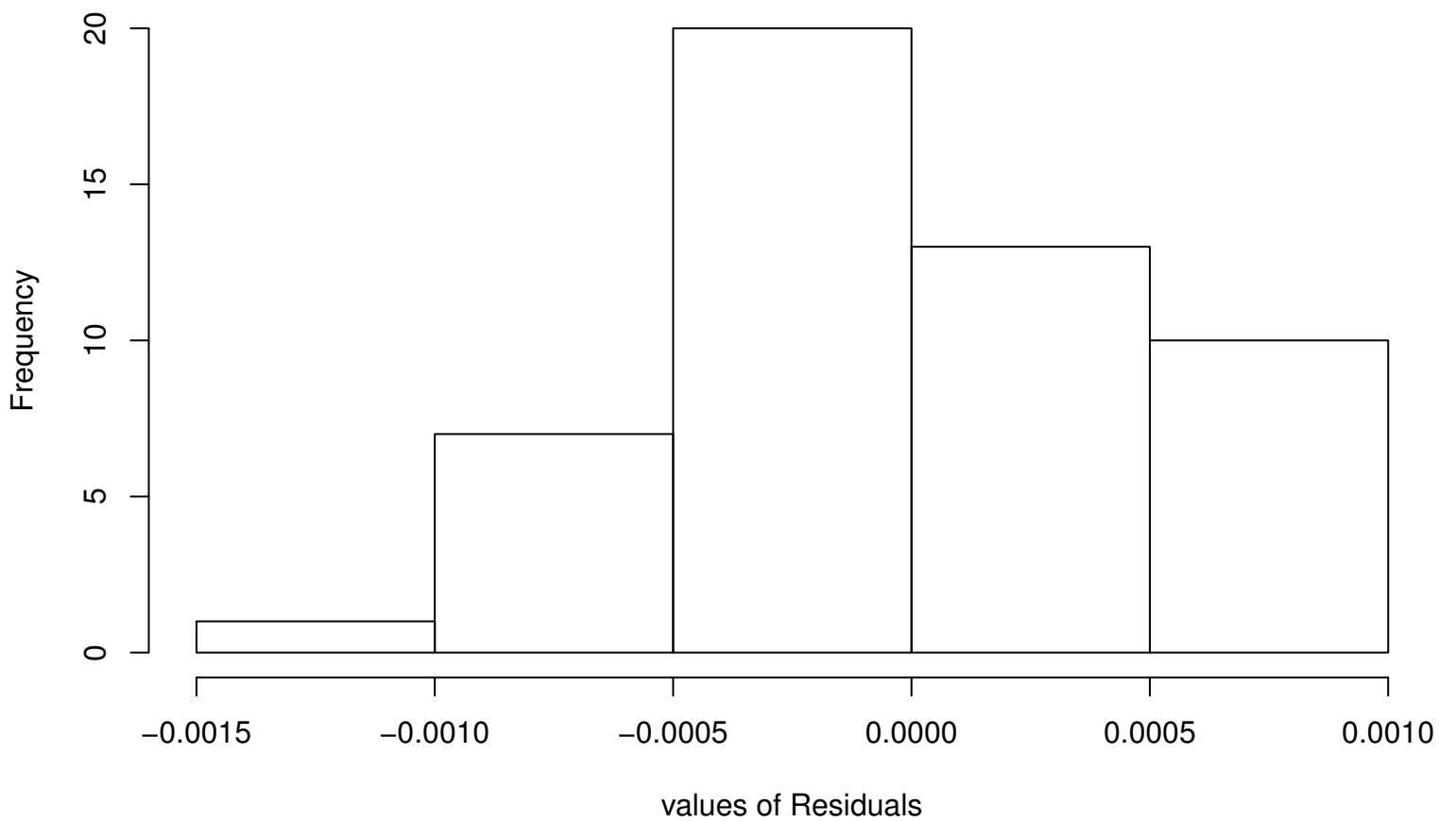
Residual Histogram
