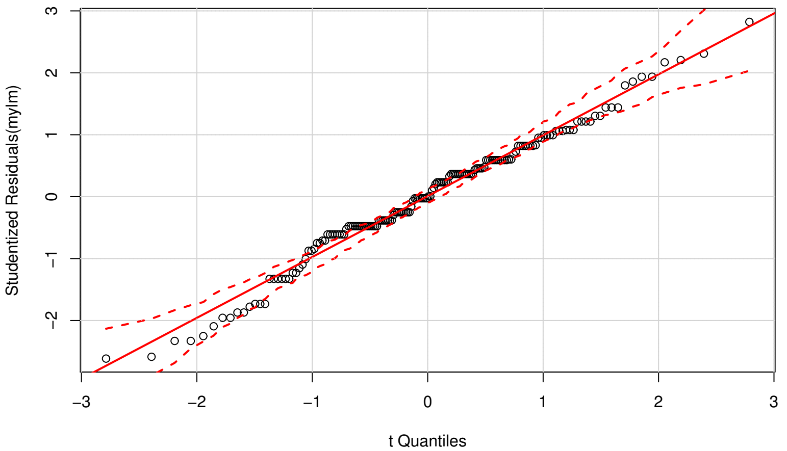
QQ Plot
