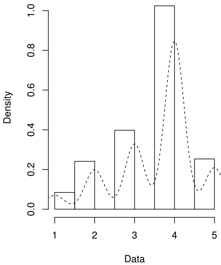
Empirical density
