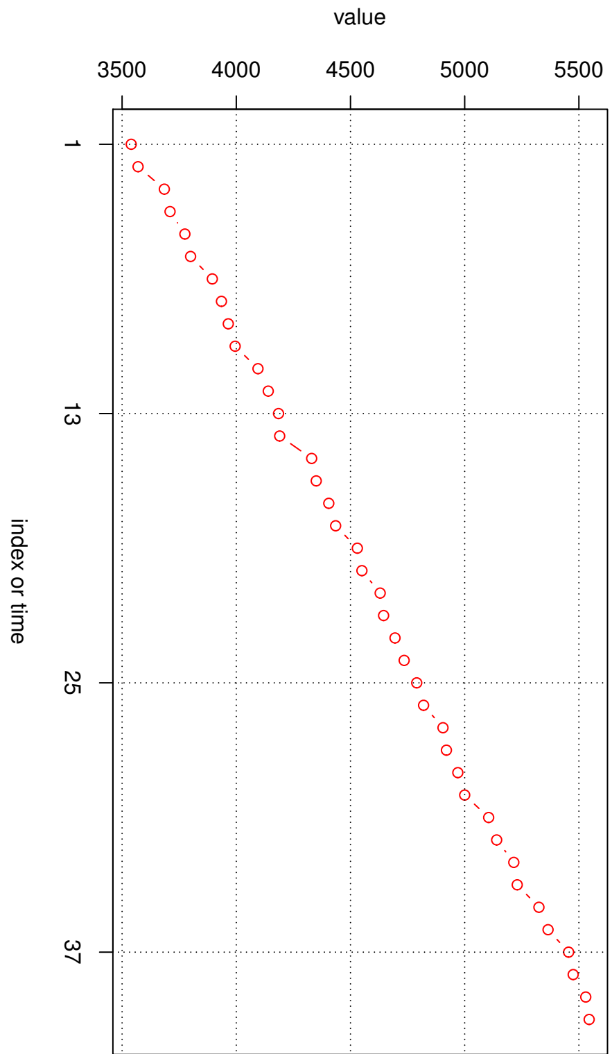
Univariate Data
