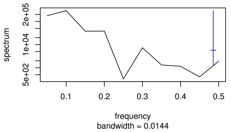
Standardized Residuals
