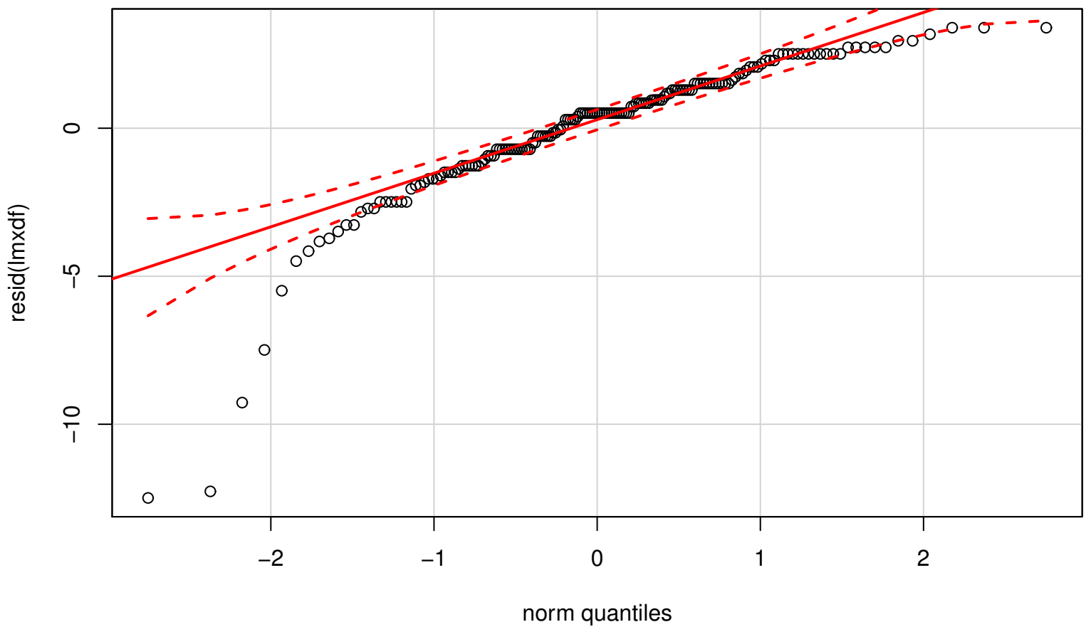
QQplot of Residuals of Fit
