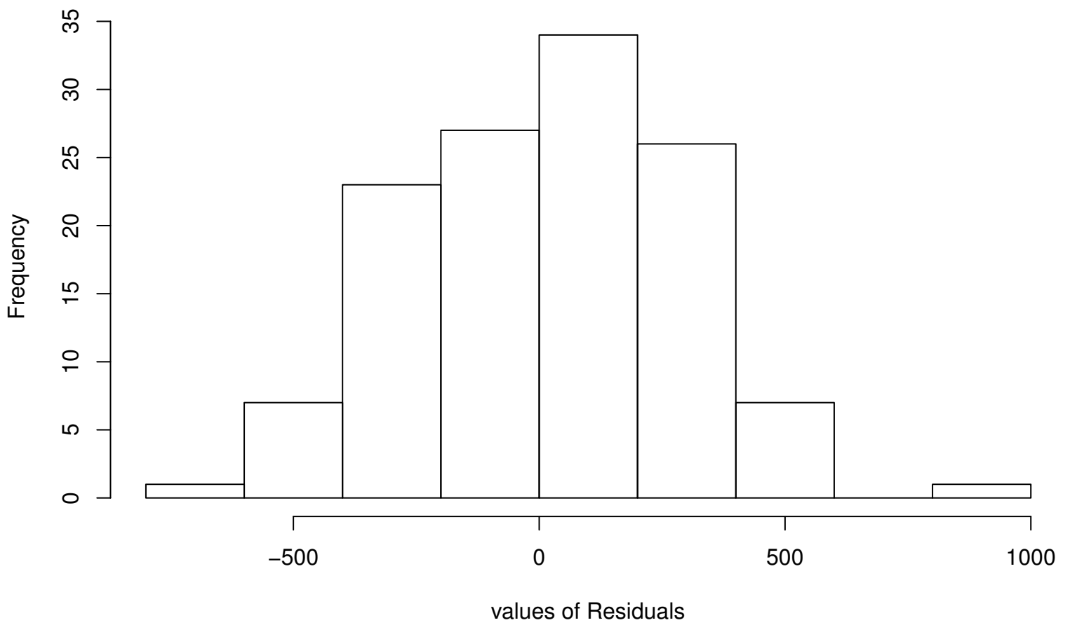
Residual Histogram
