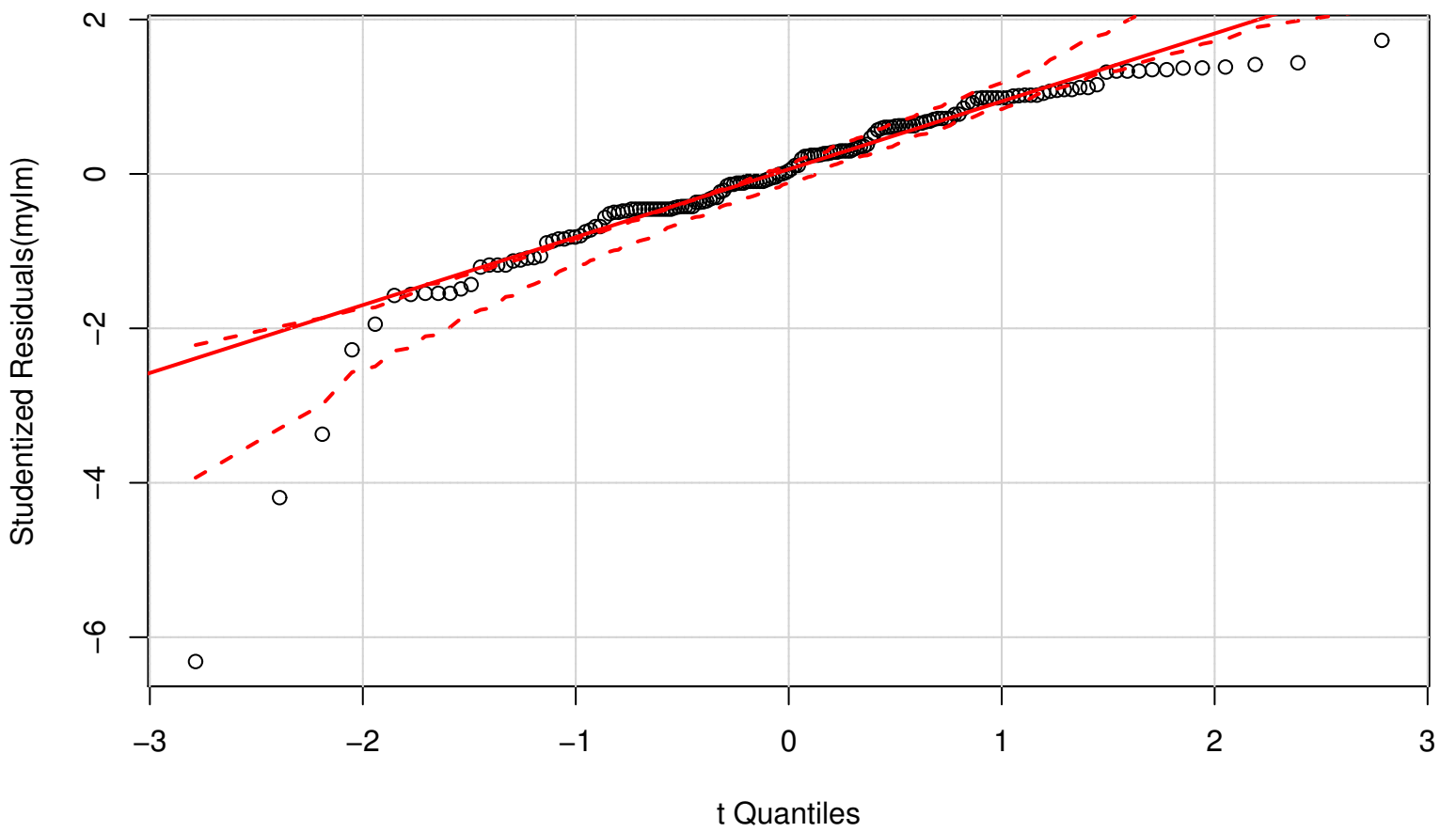
QQ Plot
