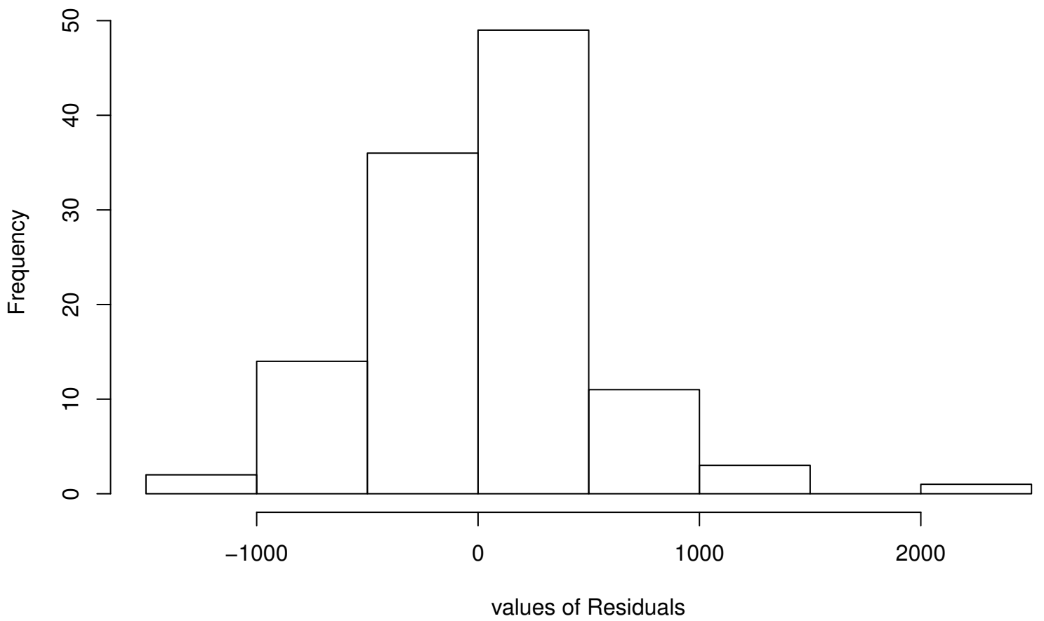
Residual Histogram
