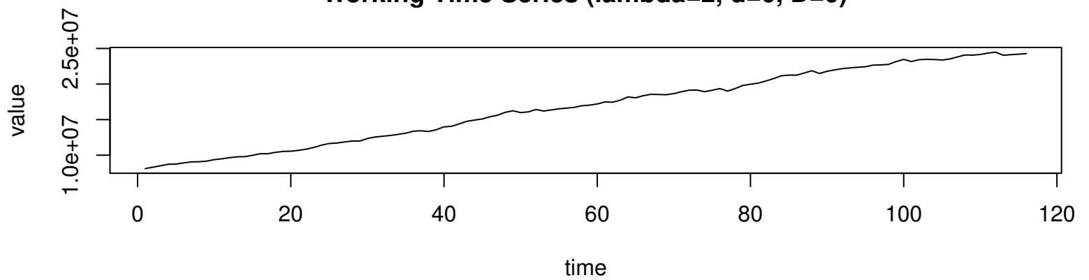
Working Time Series (lambda=2, d=0, D=0)
