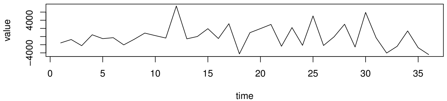
Working Time Series (lambda=1.4, d=1, D=2)
