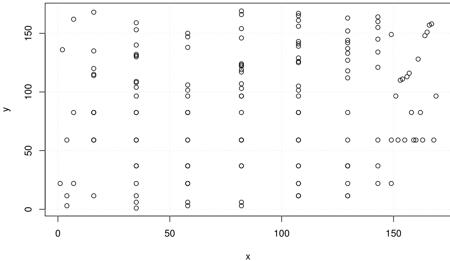
Scatterplot of Ranks
