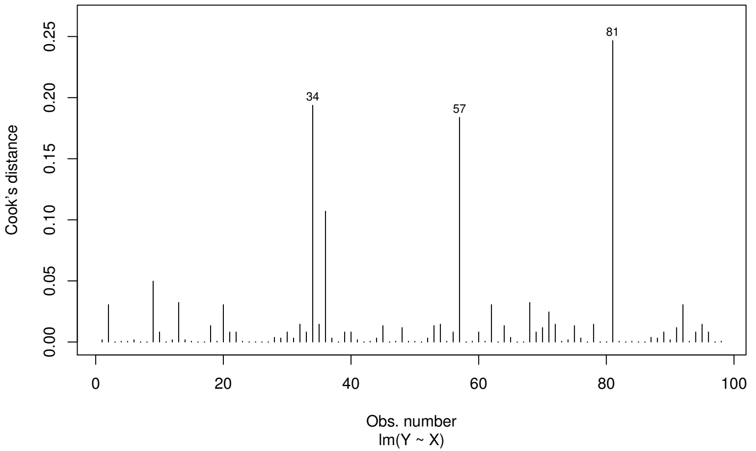
Cook's distance
