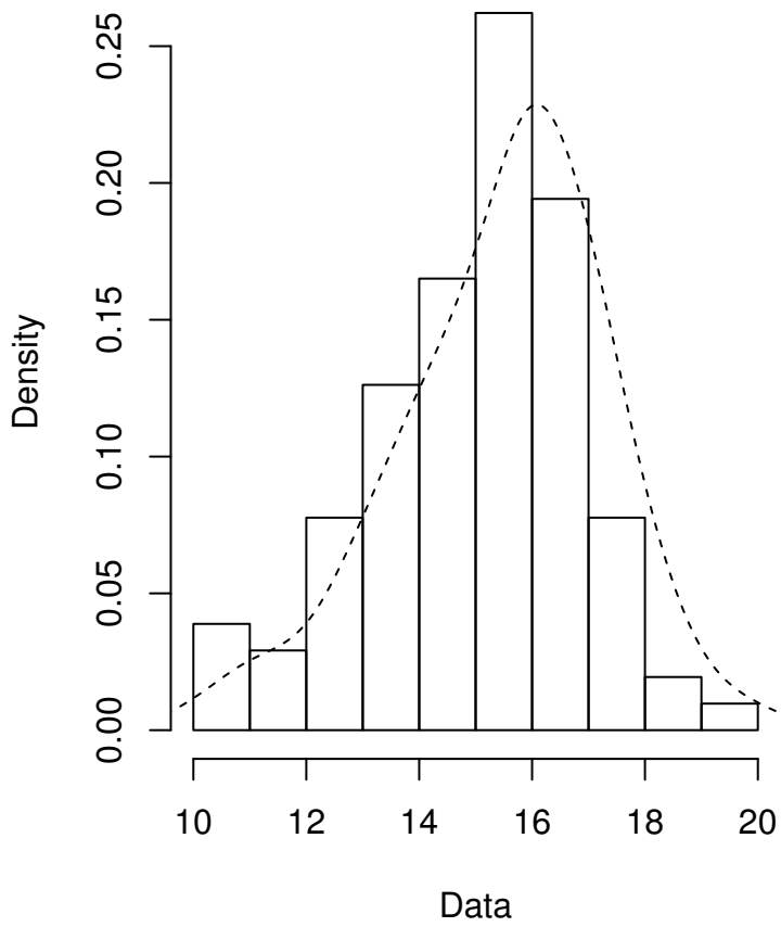
Empirical density
