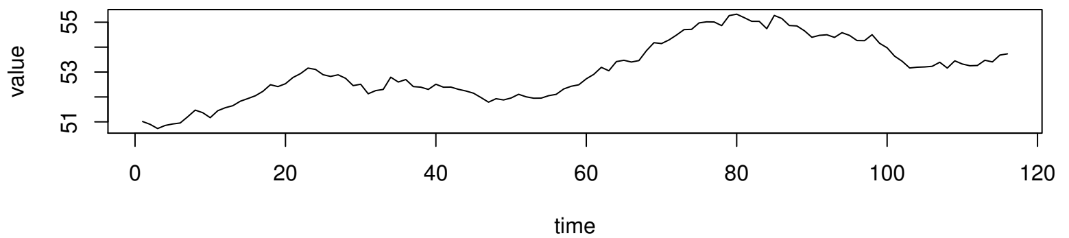
Working Time Series (lambda=0.4, d=0, D=0)
