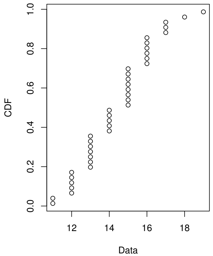
Cumulative distribution
