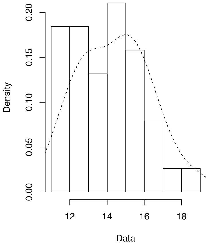
Empirical density
