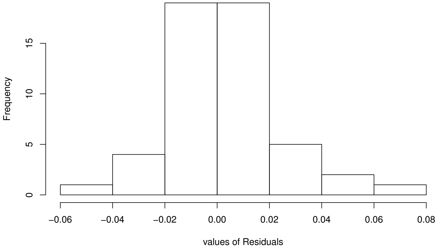
Residual Histogram
