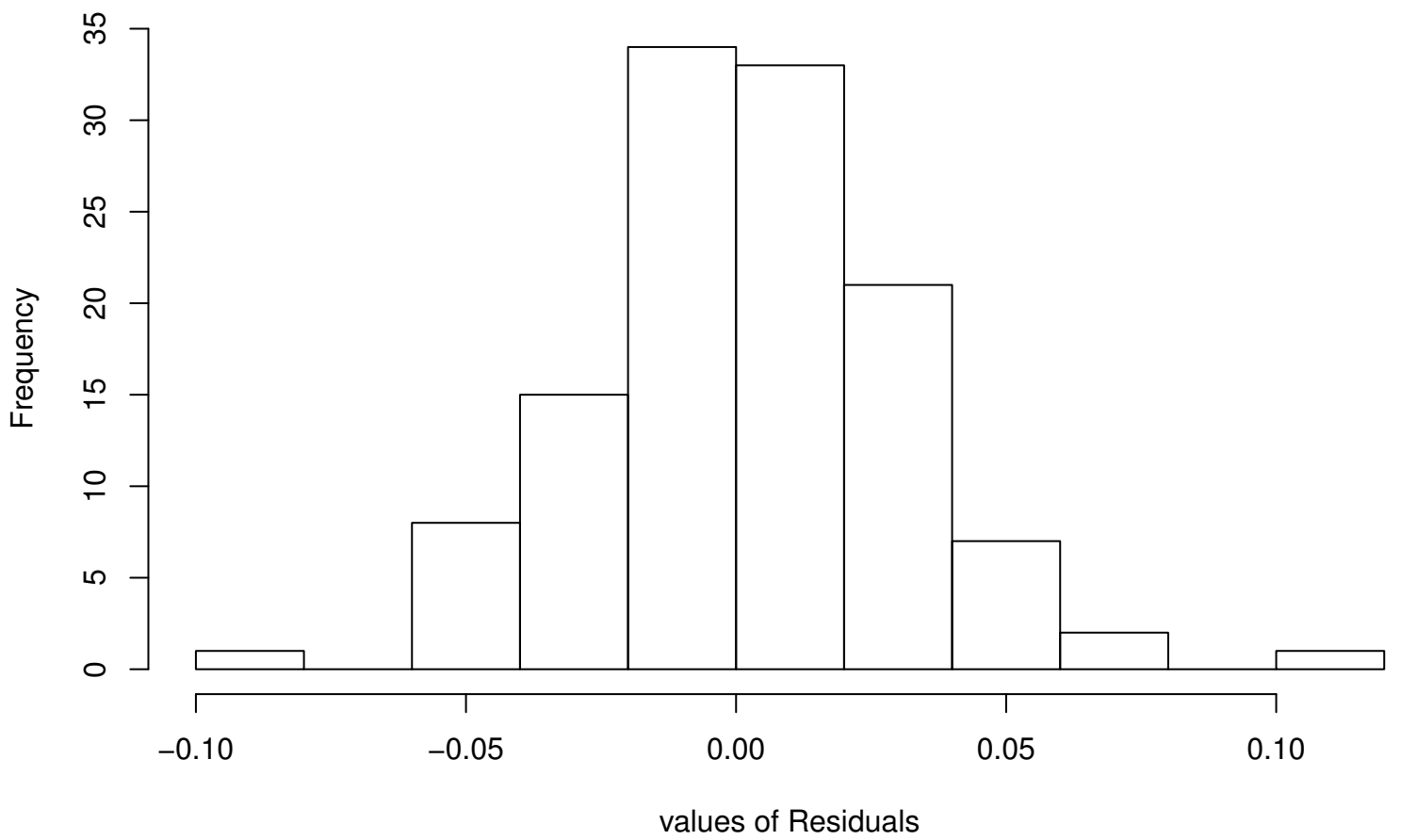
Residual Histogram
