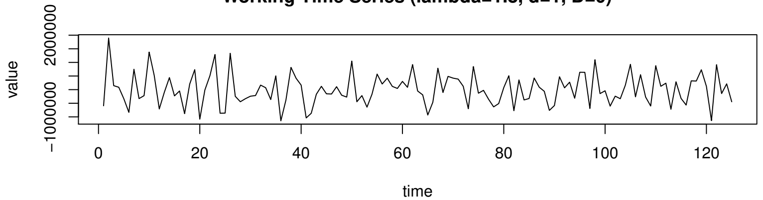
Working Time Series ( \lambda=1.8 , d=1 , D=0 )
