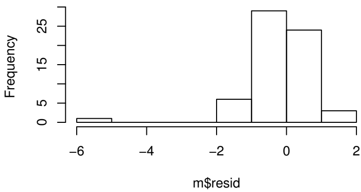
Residual Histogram
