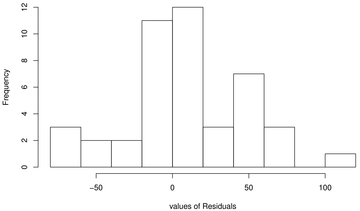
Residual Histogram
