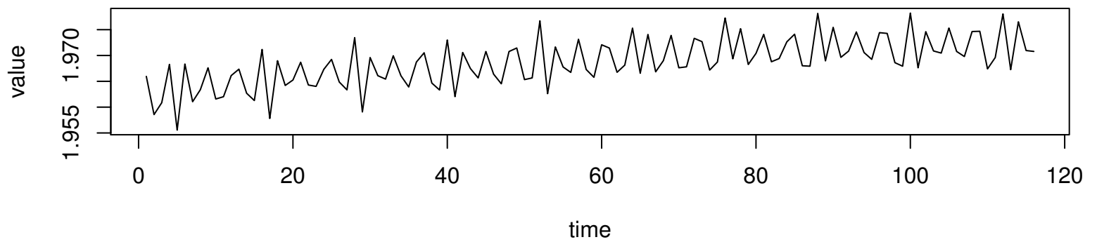
Working Time Series ( \lambda=-0.5 , d=0 , D=0 )
