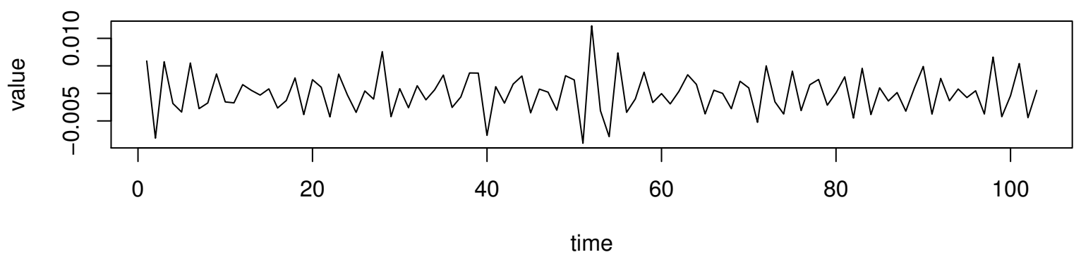
Working Time Series ( \lambda=-0.4 , d=1 , D=1 )
