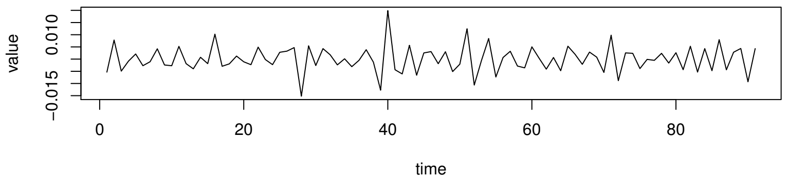
Working Time Series ( \lambda=-0.4 , d=1 , D=2 )
