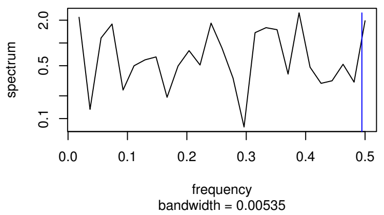
Standardized Residuals
