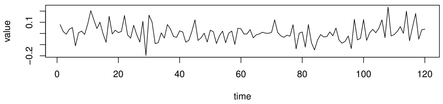
Working Time Series ( \lambda=-0.3 , d=0 , D=1 )
