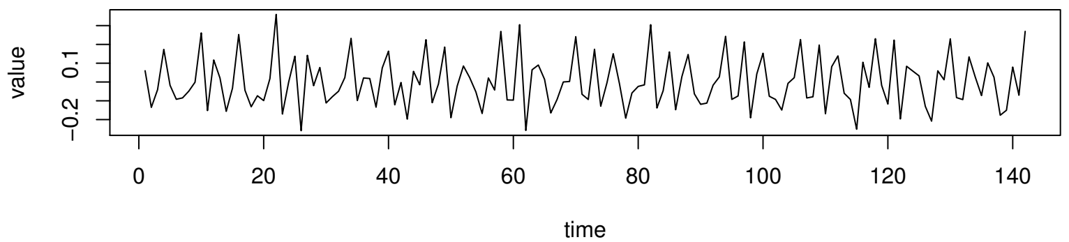
Working Time Series ( \lambda=0 , d=2 , D=0 )
