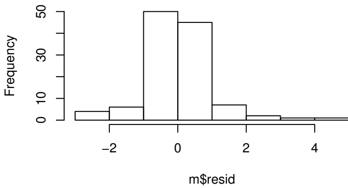
Residual Histogram
