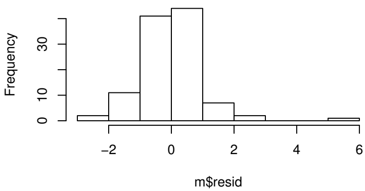
Residual Histogram
