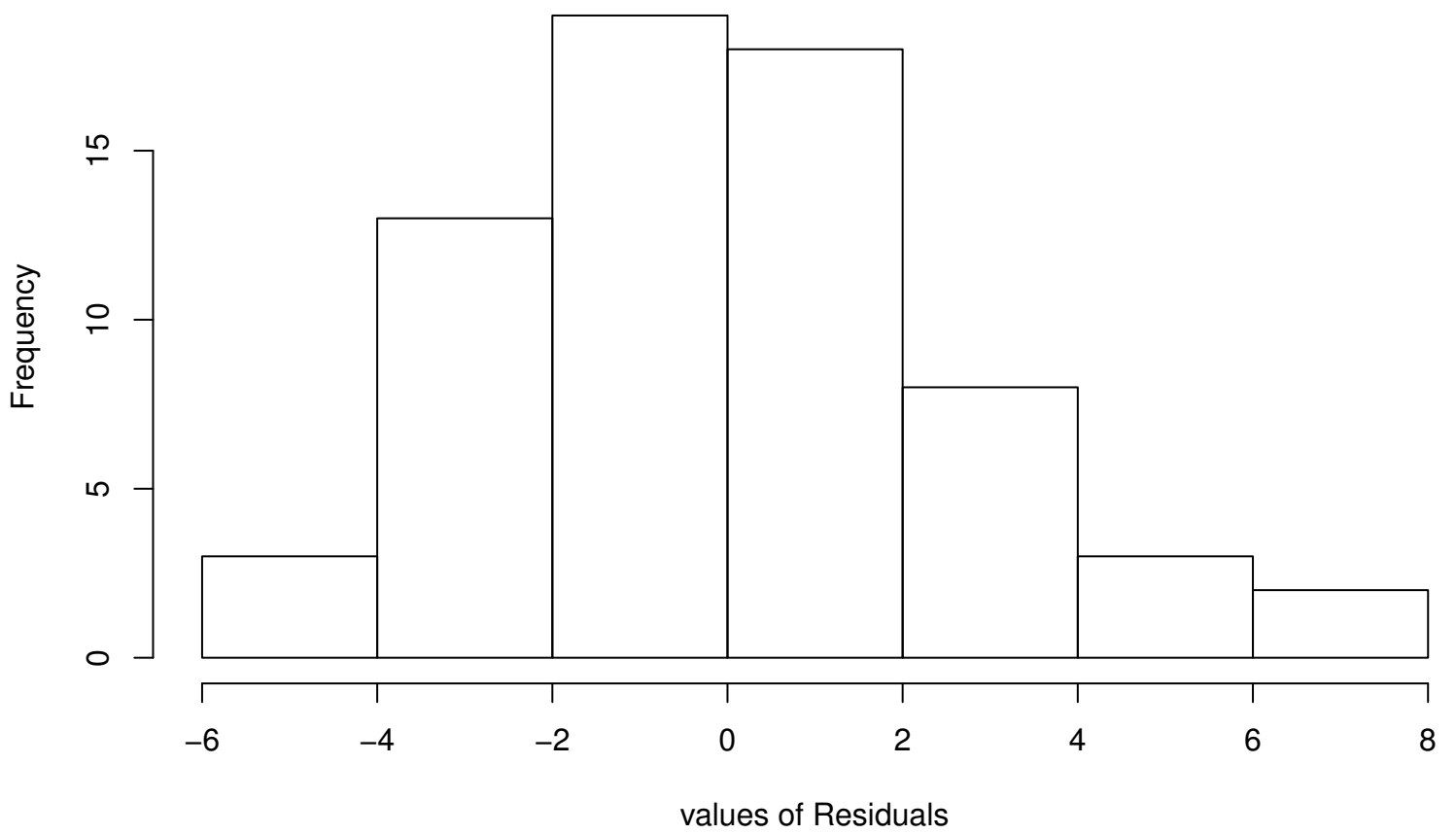
Residual Histogram
