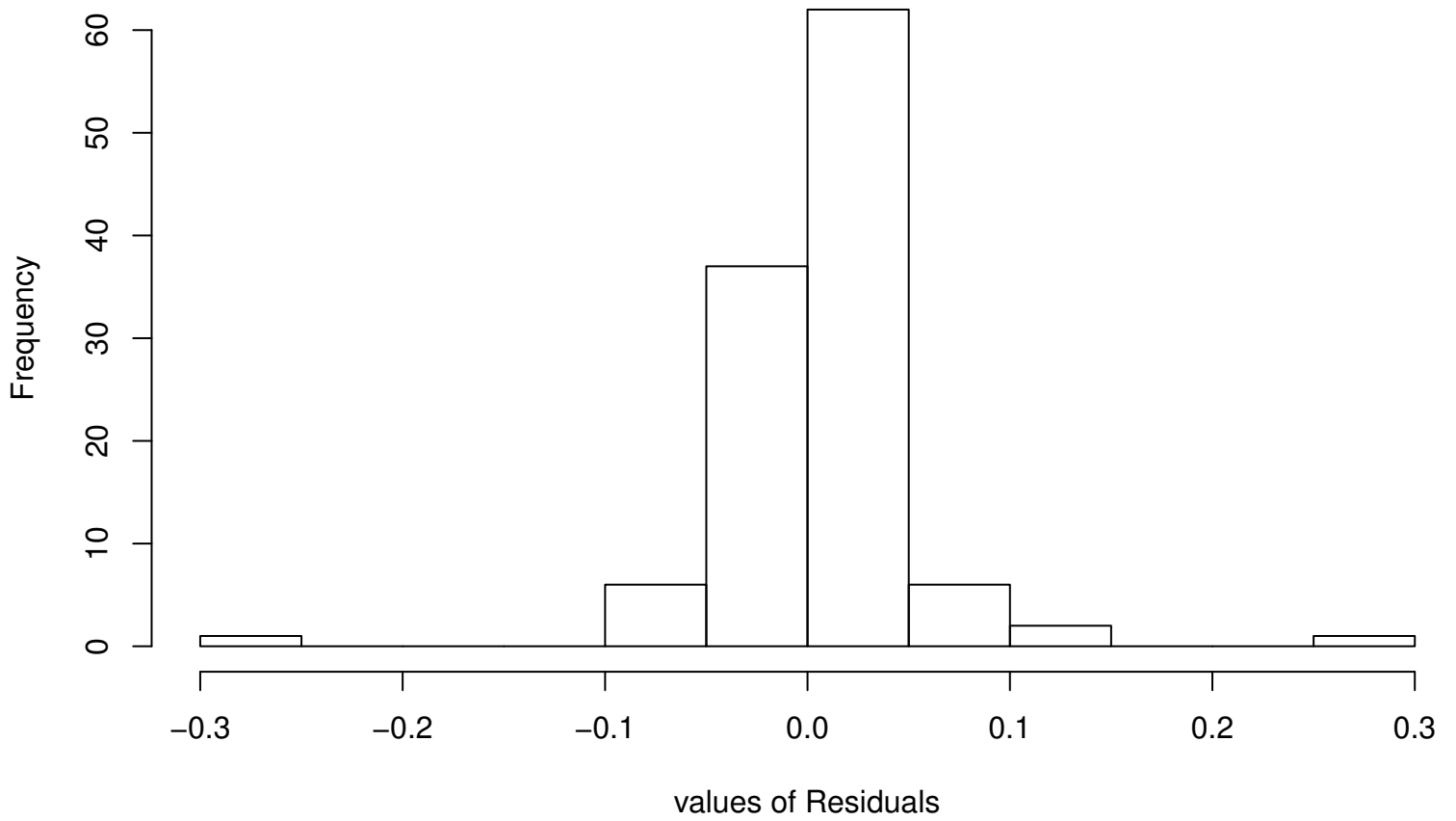
Residual Histogram
