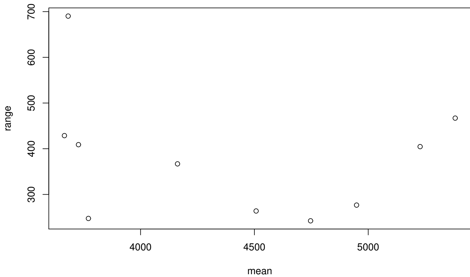
Range–Mean Plot
