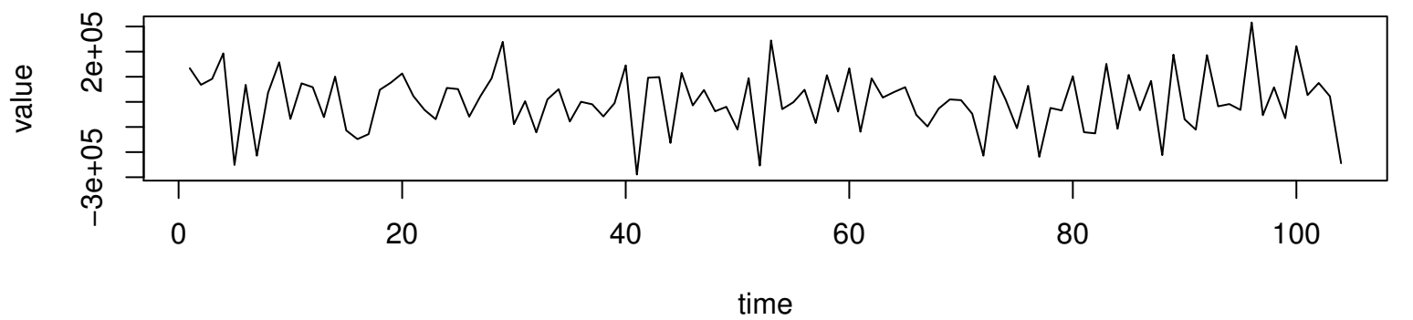
Working Time Series ( \lambda=2 , d=1 , D=1 )
