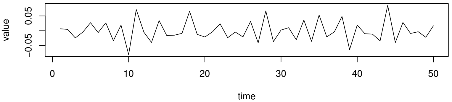
Working Time Series ( \lambda=-0.3 , d=1 , D=0 )
