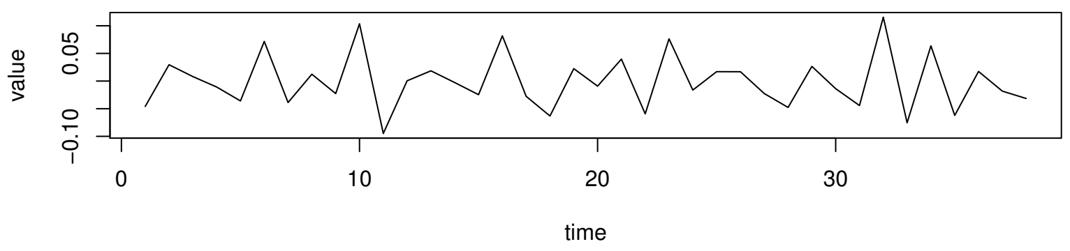
Working Time Series ( \lambda=-0.3 , d=1 , D=1 )
