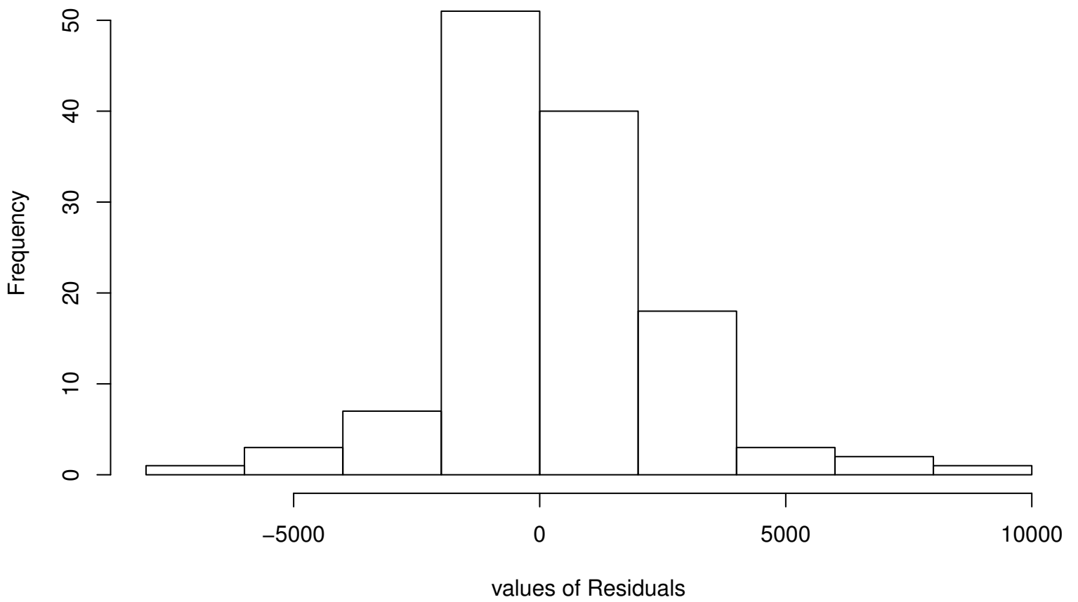
Residual Histogram
