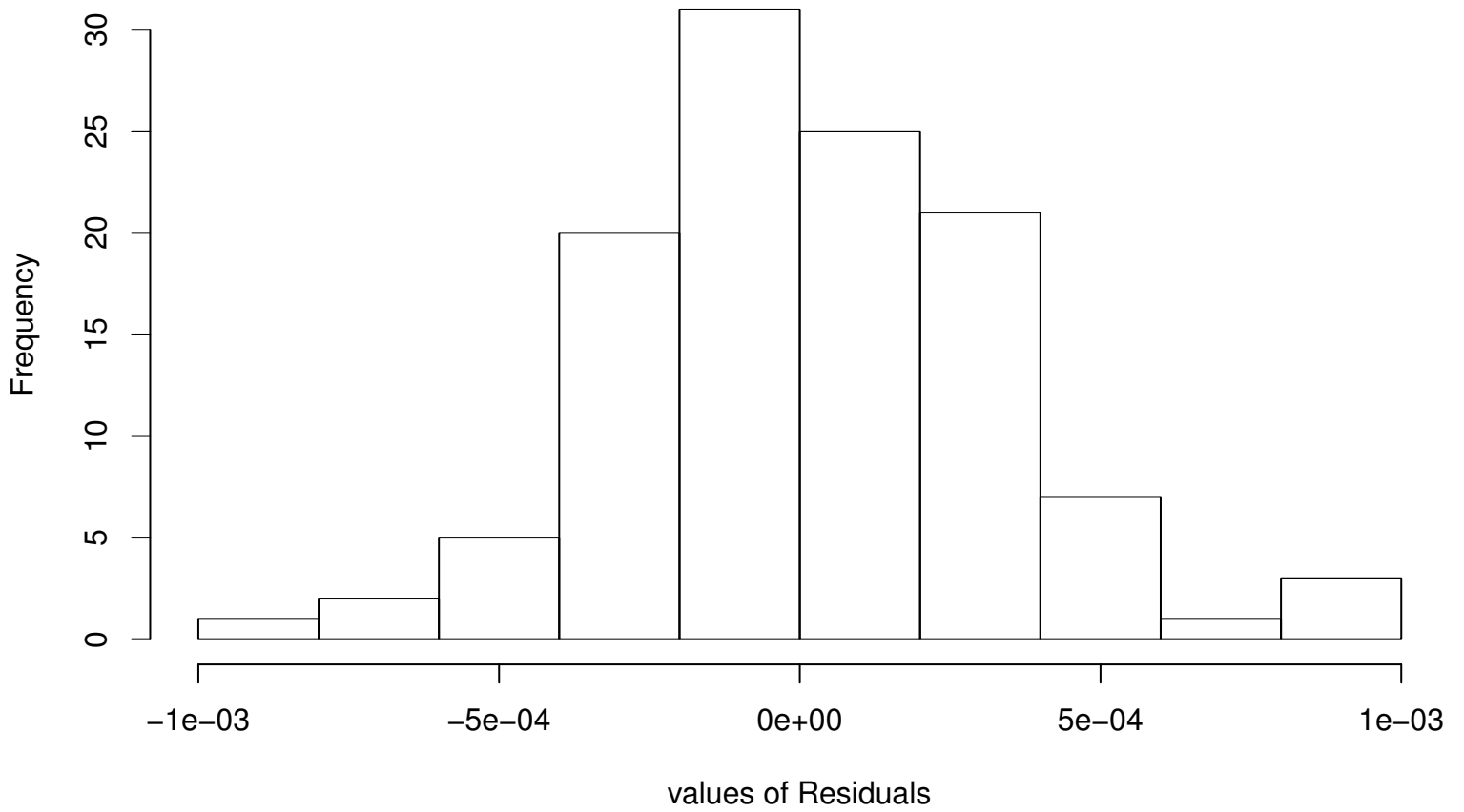
Residual Histogram
