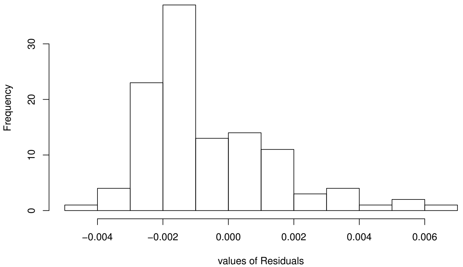
Residual Histogram
