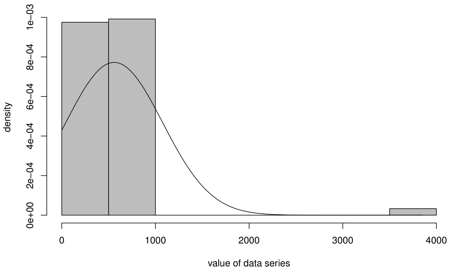
Histogram and Fitted Normal Density
