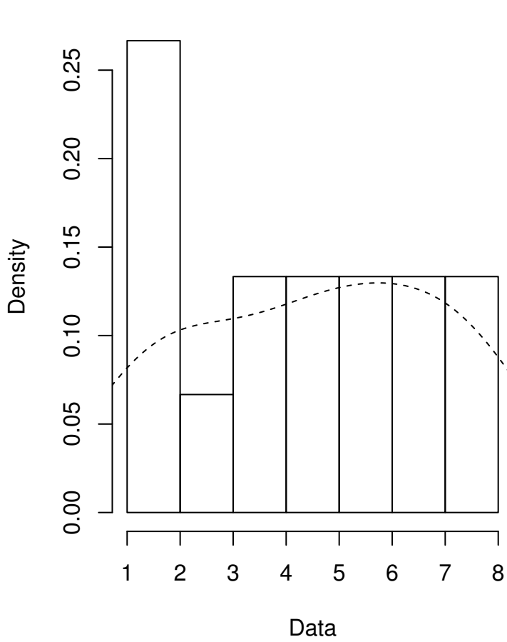
Empirical density
