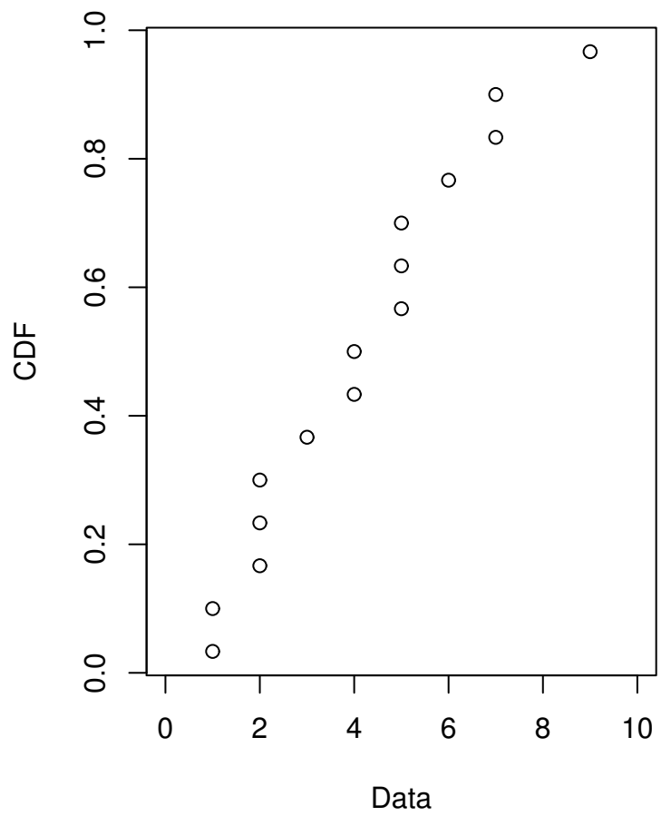
Cumulative distribution
