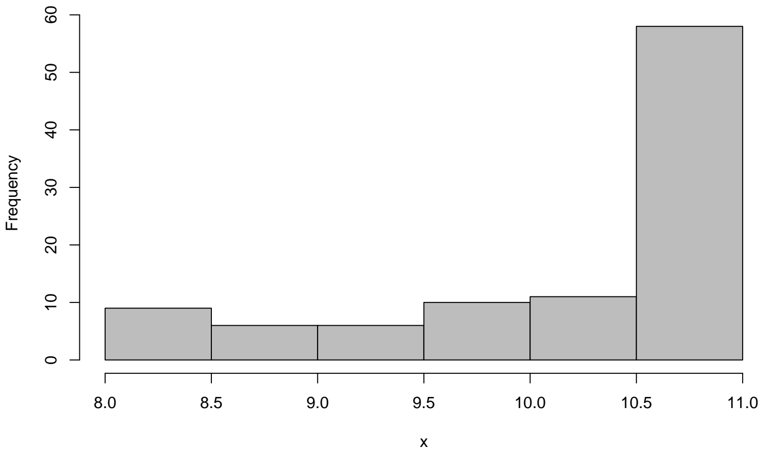
Histogram
