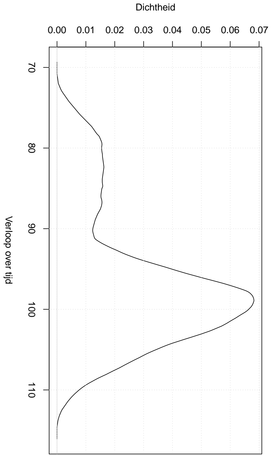
Triangular Kernel
